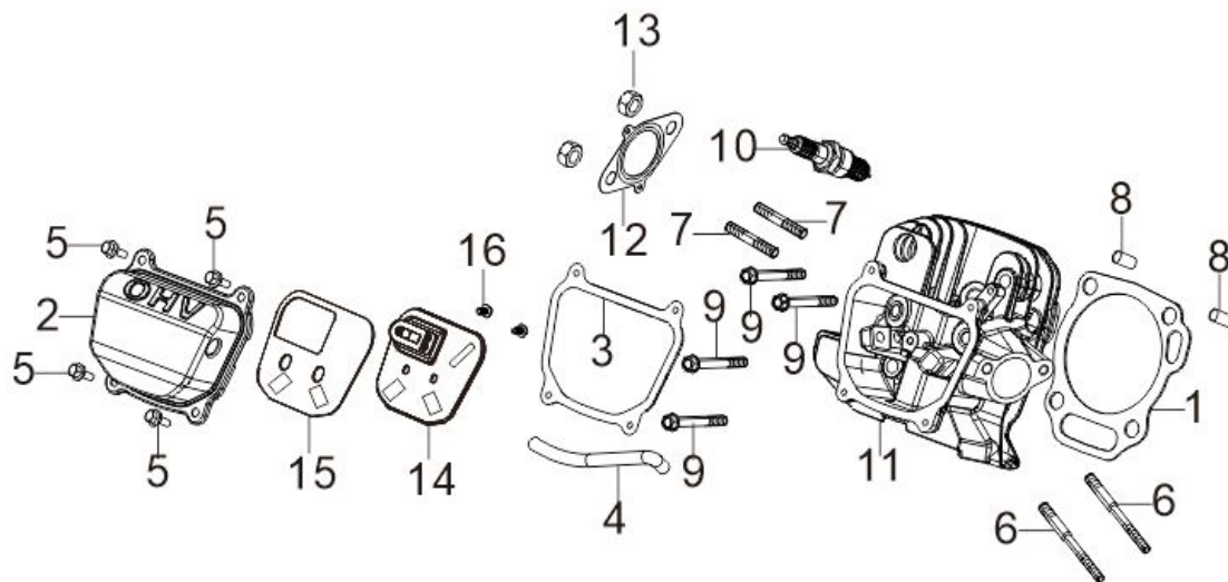
FIG.3 HEAD SUBASSEMBLY, CYLINDER / PLUG,SPARK 气缸头部件/火花塞 (E03)
