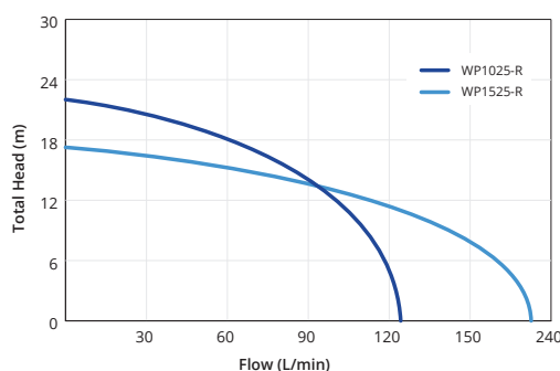
Performance Curve
