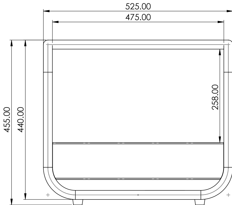
SIDE VIEW
