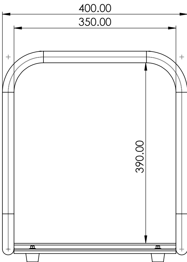
SIDE VIEW
