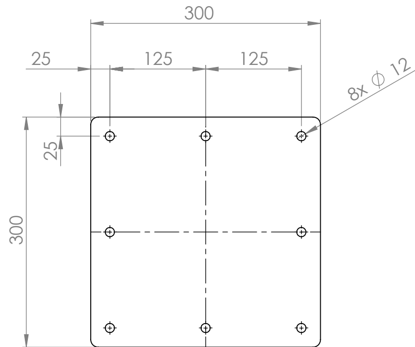
Footprint
